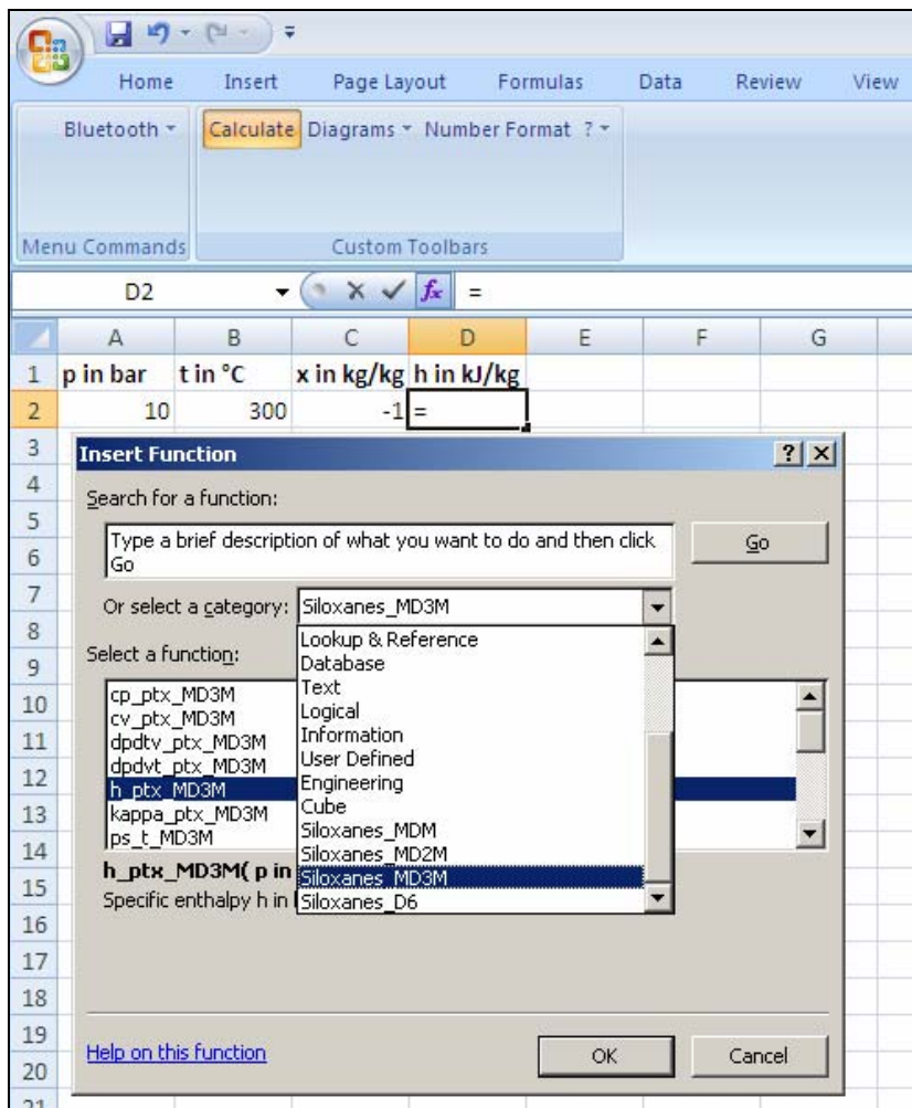
Figure 2.23: Choice of library and function name
