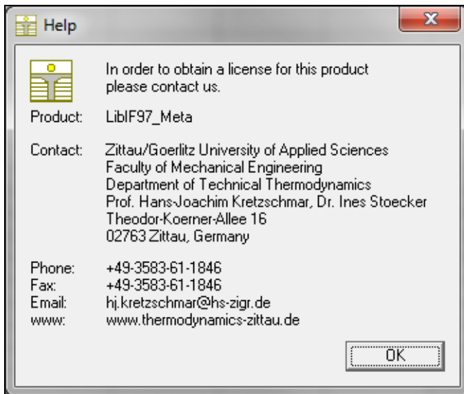
Figure 2.7 "Help" window
