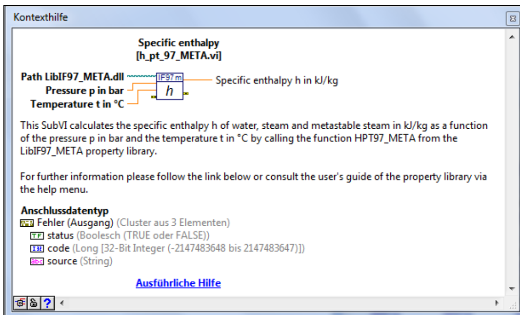
Figure 2.2 Context help window of the function h_pt_97_META.vi
